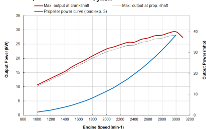
3JH40 Output Power curve
